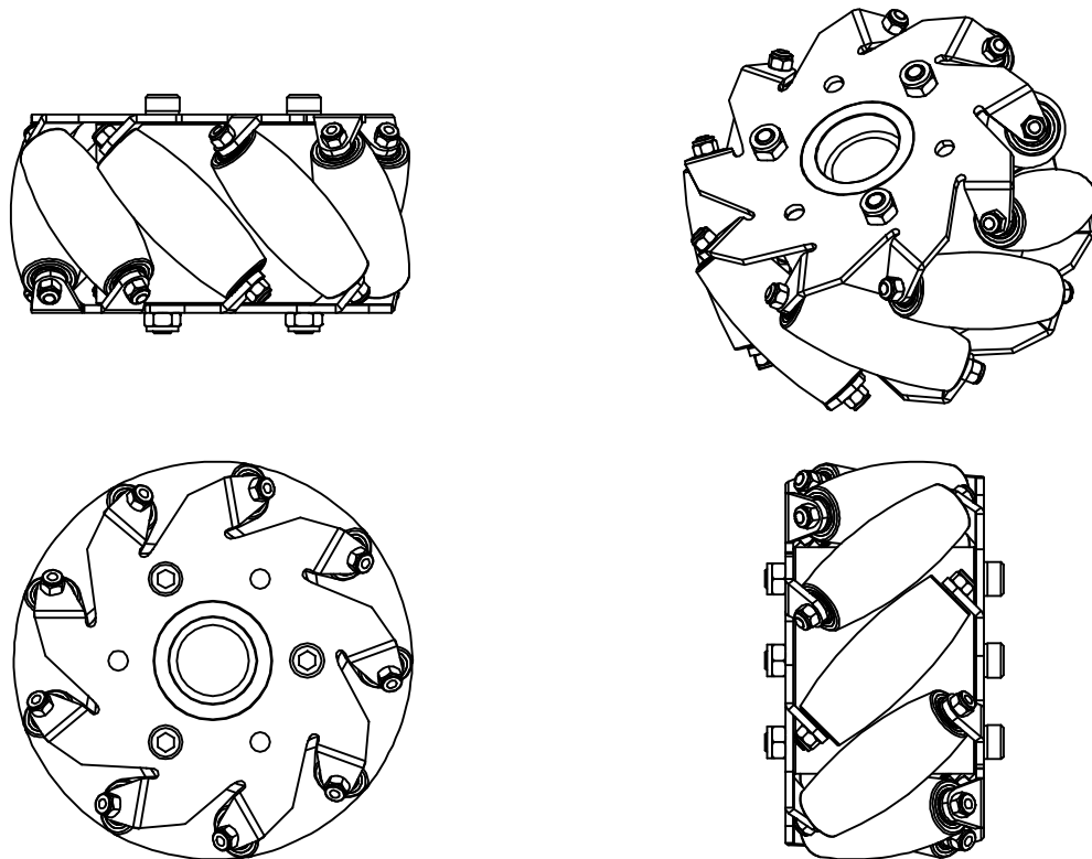
100mm Mecanum Wheel Right
