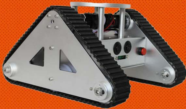
KR0002 Tri-Track Tank Robot Kit with Ultrasonic Sensors
